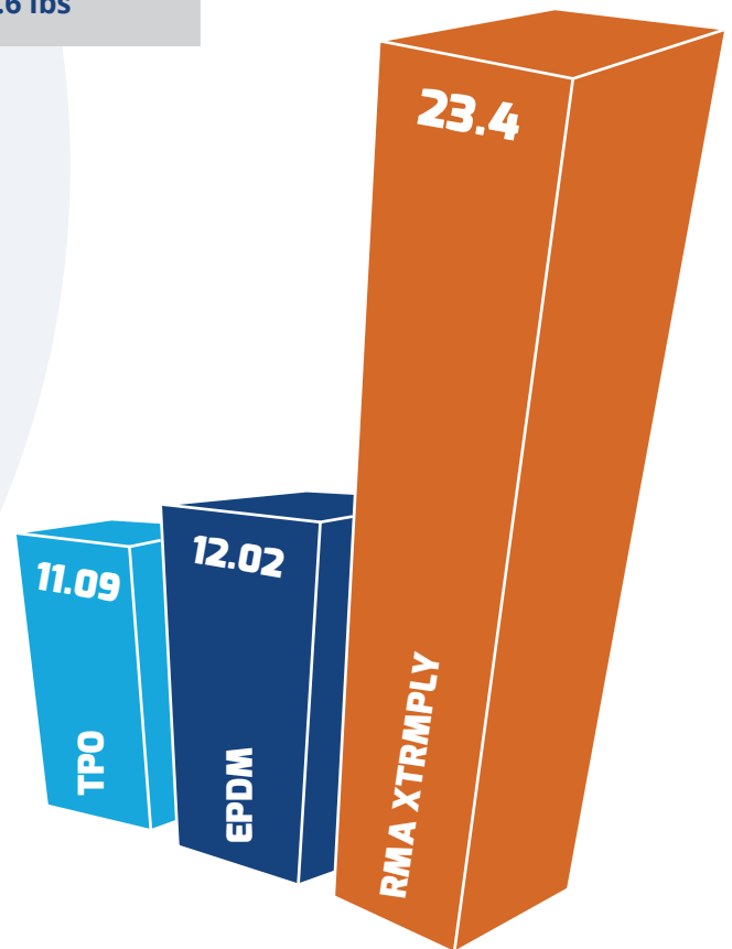
SCREW PUNCTURE TEST
